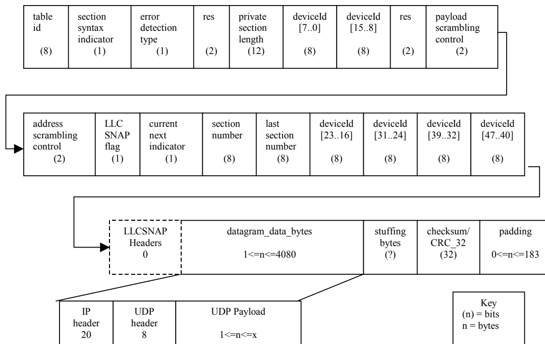
Figure 6.8 DSM-CC addressable section syntax.
