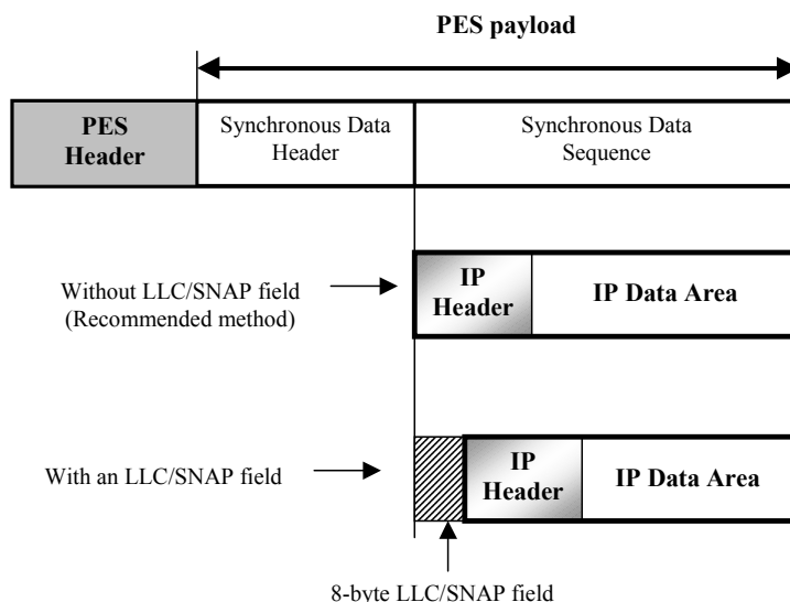
Figure 6.11 Encapsulation of IP packets for synchronous data streaming using PES frames.
