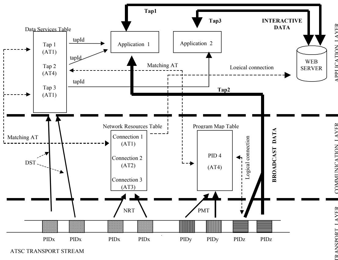
Figure 8.2 Service description block diagram..
