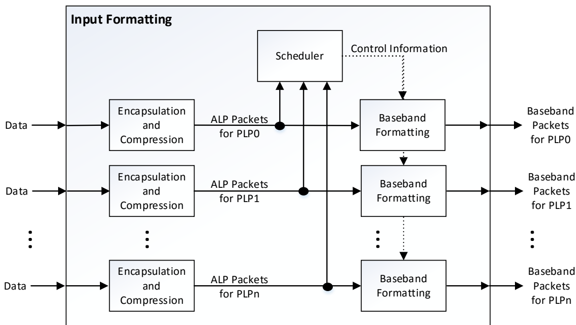
Figure 5.1 Block diagram of input formatting.
