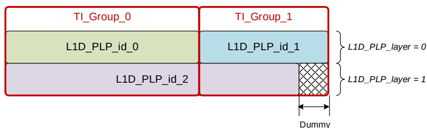
Figure 7.23 Example Insertion of Enhanced Layer dummy cells when the HTI mode is used with Layered-Division Multiplexing.
