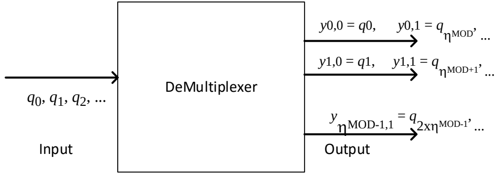
Figure 6.11 De-multiplexing of bits into sub-streams.
