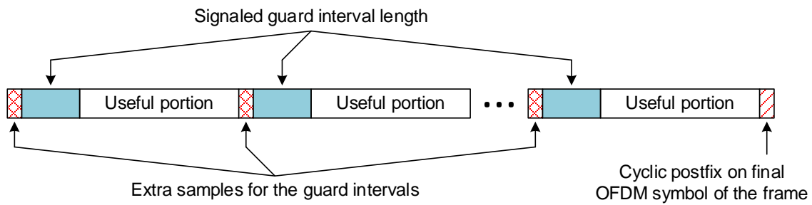
Figure 8.4 Illustration of the assignment of extra samples to the guard interval of each non-Preamble OFDM symbol in a frame.
