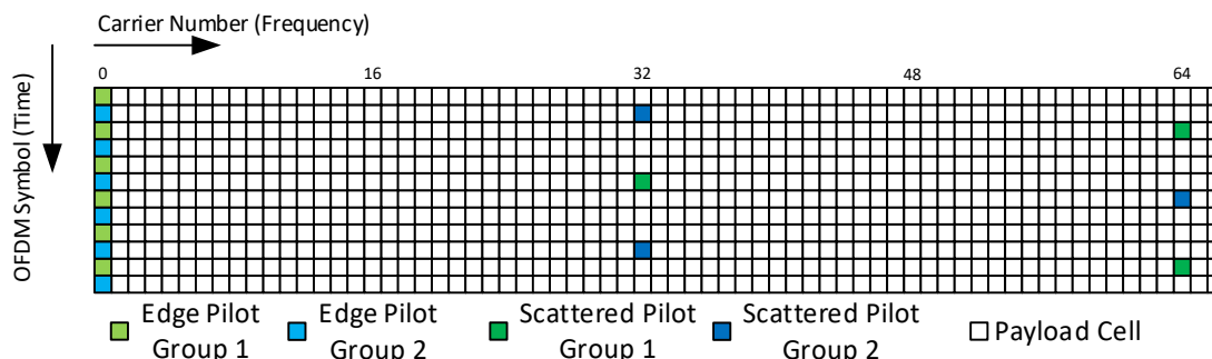
Figure L.11.28 MIMO pilot scheme MP32_4 for null pilot encoding.
