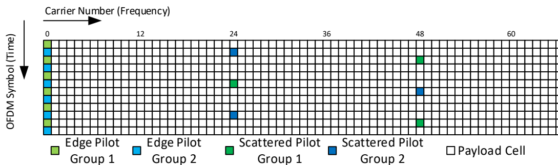
Figure L.11.26 MIMO pilot scheme MP24_4 for null pilot encoding.
