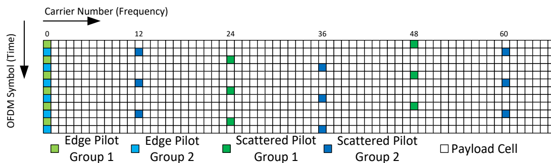
Figure L.11.10 MIMO pilot scheme MP12_4 for Walsh-Hadamard pilot encoding.
