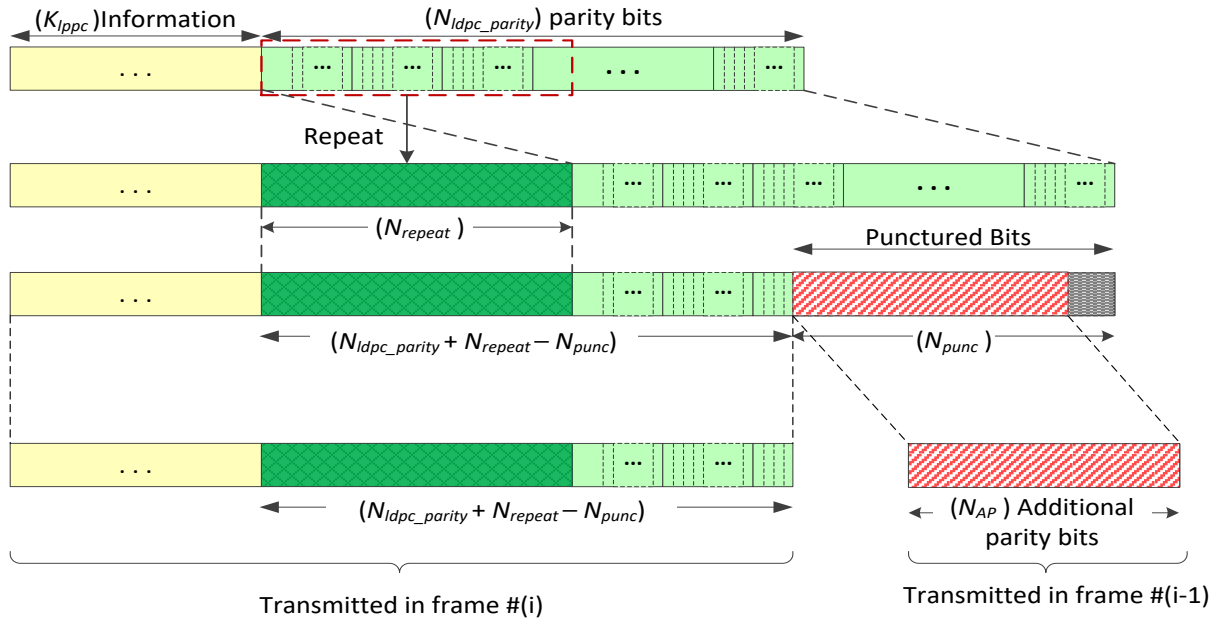
Figure 6.32 Additional parity generation for L1-Detail signaling ( N_{AP} \leq N_{punc} ).
