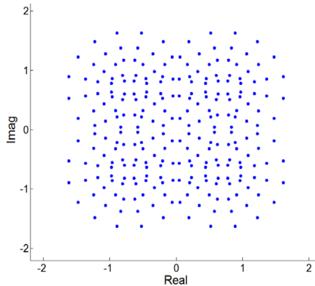
Figure 6.17 Example combined constellation after normalization.
