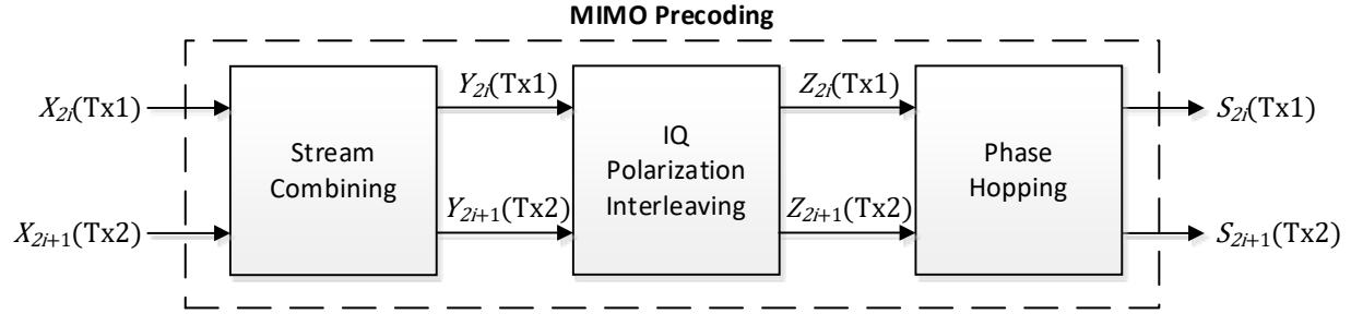
Figure L.7.2 Detailed MIMO precoding block diagram.
