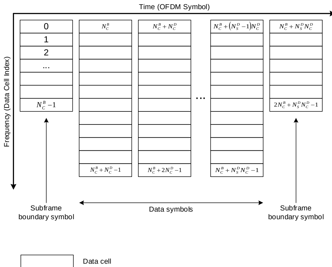
Figure 7.13 Data cell addressing when a Preamble symbol is not associated with a subframe.
