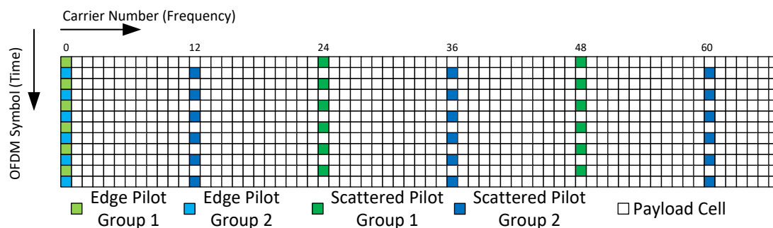
Figure L.11.9 MIMO pilot scheme MP12_2 for Walsh-Hadamard pilot encoding.
