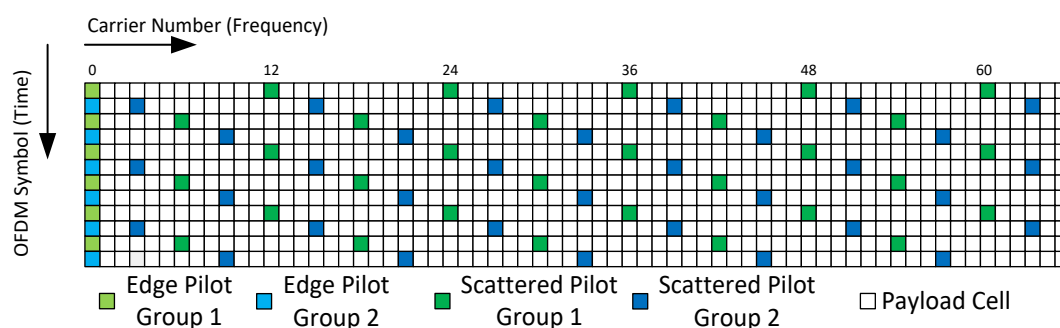
Figure L.11.2 MIMO pilot scheme MP3_4 for Walsh-Hadamard pilot encoding.
