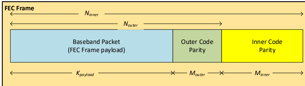
Figure A.4.1 FEC coding.
