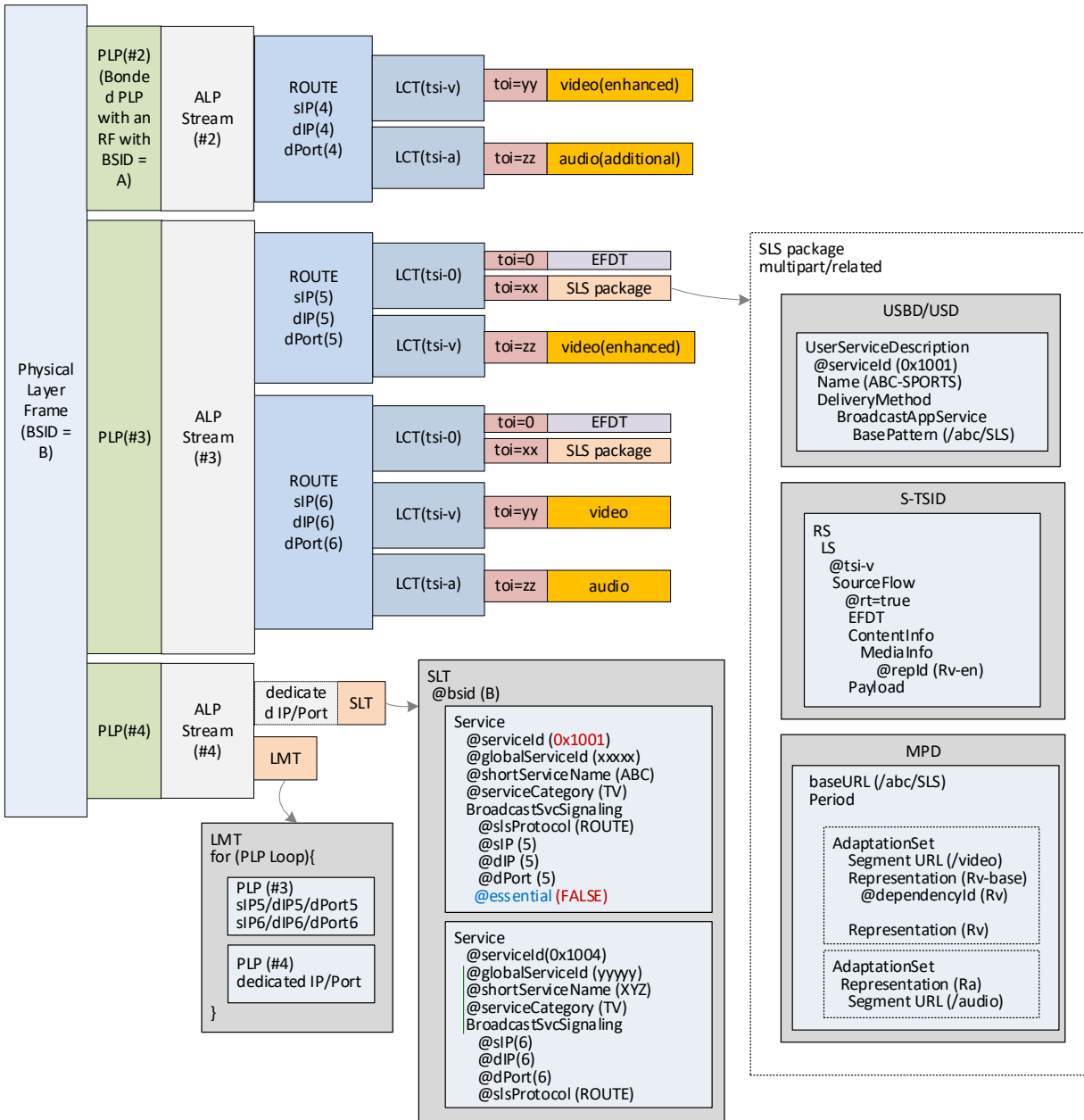
Figure B.14.2 Portions of a Service delivered in multiple RF channels with channel bonding – Case #1: essential portion is delivered in non-bonded PLP(s) (second channel).
