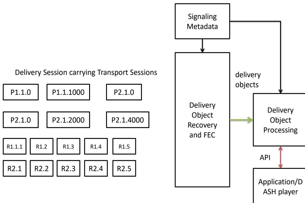
Figure A.4.8 ROUTE receiver with FEC.
