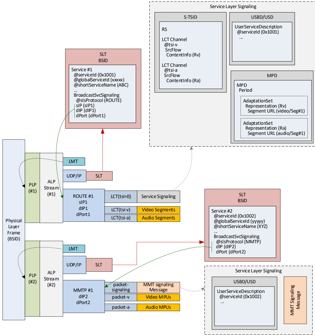
Figure B.11.1 Multiple SLTs.
