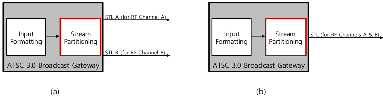
Figure 9.7 Channel Bonding operation modes in a Broadcast Gateway: (a) Sending two outer Tunnel Data Streams, and (b) Sending one outer Tunnel Data Stream that carries two groups of inner Tunneled Packet Streams.
