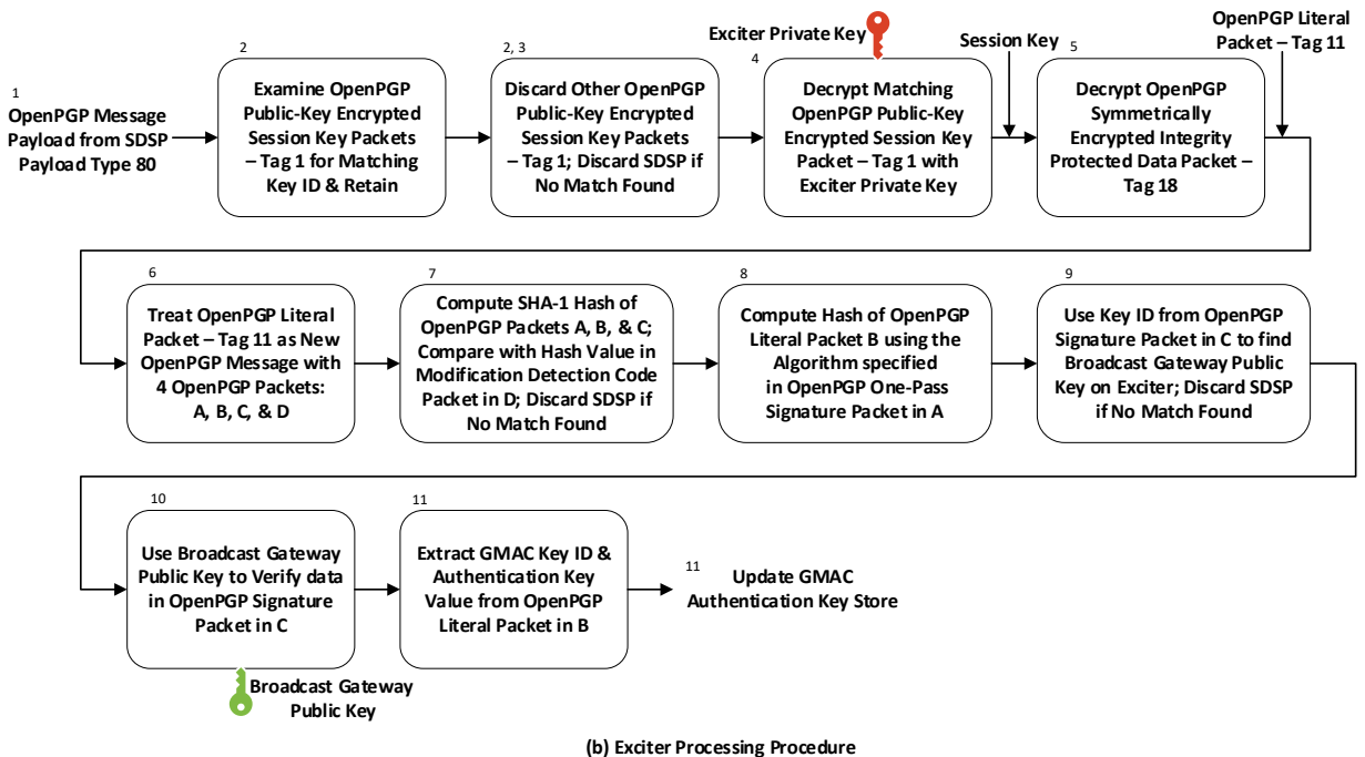
Figure 9.3 STLTP security System Authentication Key generation & distribution: (a, top) Broadcast Gateway Processing Procedure; (b, bottom) Exciter Processing Procedure.
