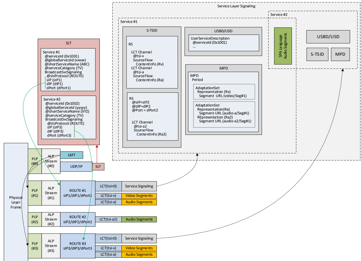
Figure B.5.1 Service acquisition in pure broadcast (multiple ROUTE sessions).
