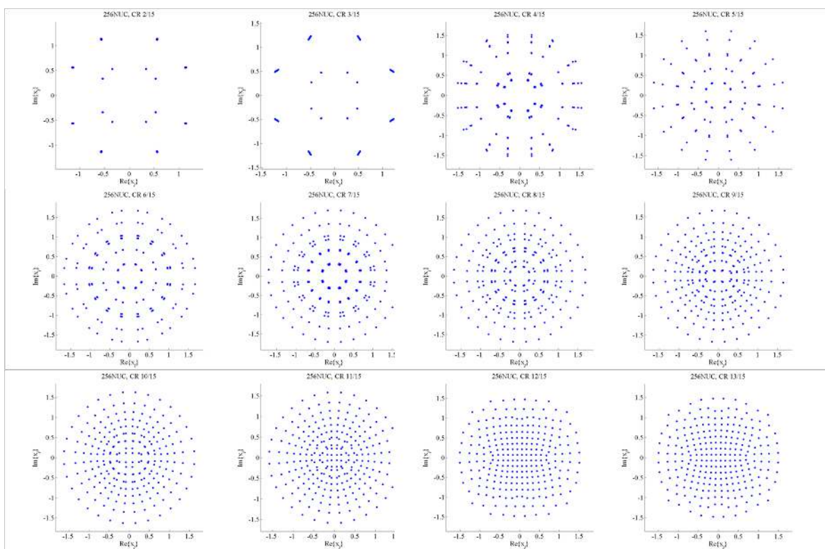
Figure C.2.4 Constellations of 256QAM.
