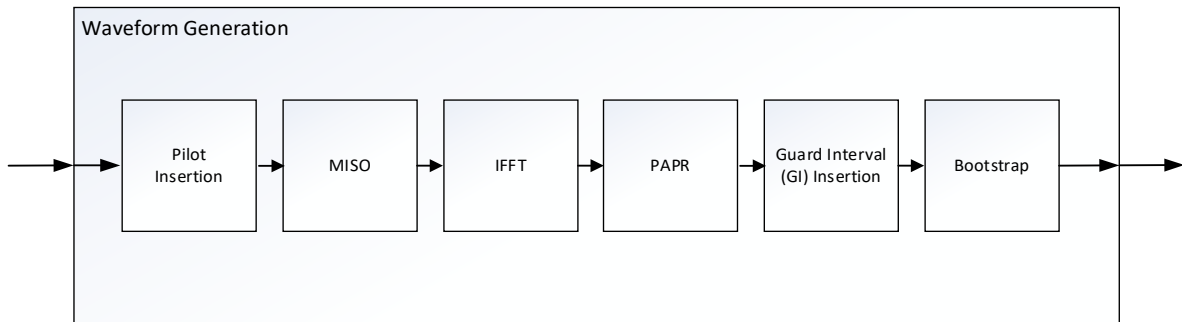
Figure 8.1 Block diagram of waveform generation.
