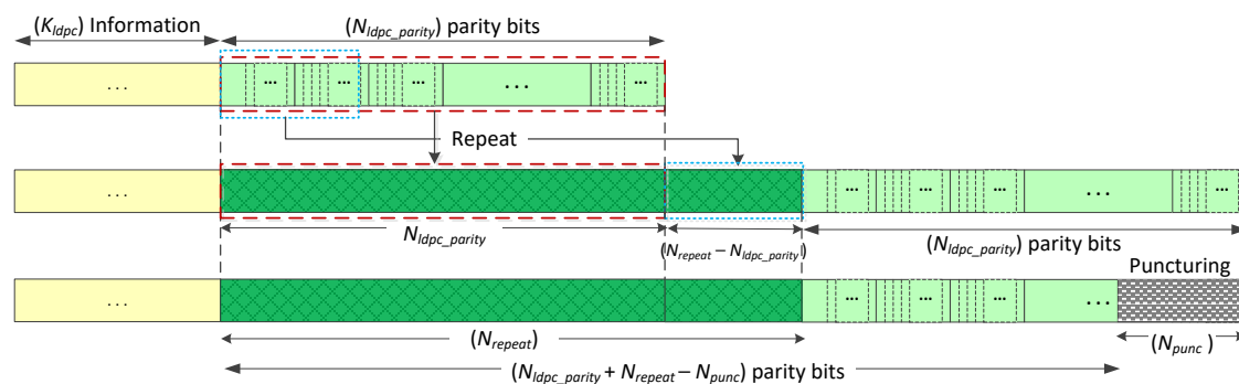
Figure 6.25 Example 2 of parity puncturing after repetition.
