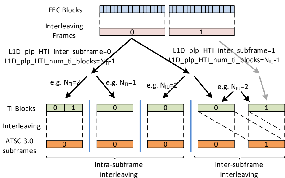
Figure 7.9 Example of HTI for L1D_plp HTI_inter_subframe = 0 and 1, and for L1D_plp HTI_num_ti_blocks = 0 and 1.
