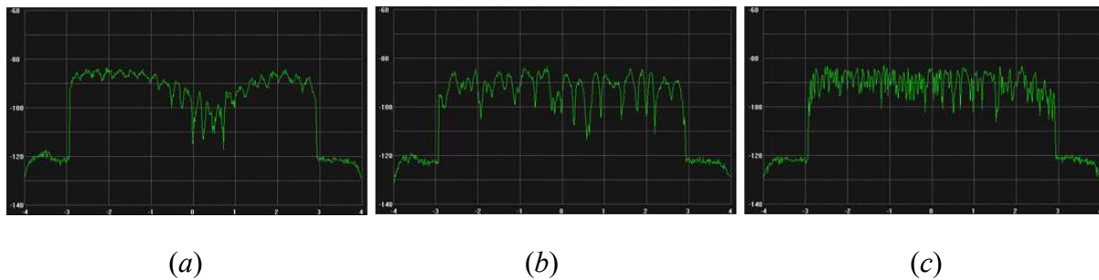
Figure 4.4 Frequency response of a two-transmitter SFN when relative delay is 0.1 \mu s: (a) No MISO, (b) MISO with 64 coefficients, and (c) MISO with 256 coefficients
