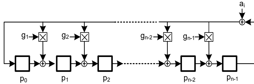
Figure 6.7 Shift register for CRC.
