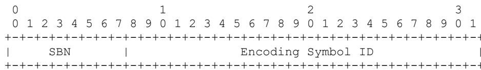
Figure A.3.4 FEC Payload ID for Repair Flows.
