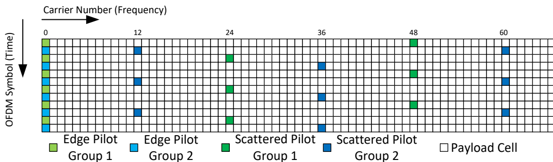
Figure L.9.10 MIMO pilot scheme MP12_4 for Walsh-Hadamard pilot encoding.
