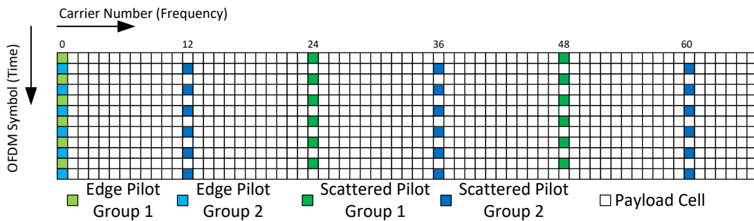
Figure L.9.9 MIMO pilot scheme MP12_2 for Walsh-Hadamard pilot encoding.
