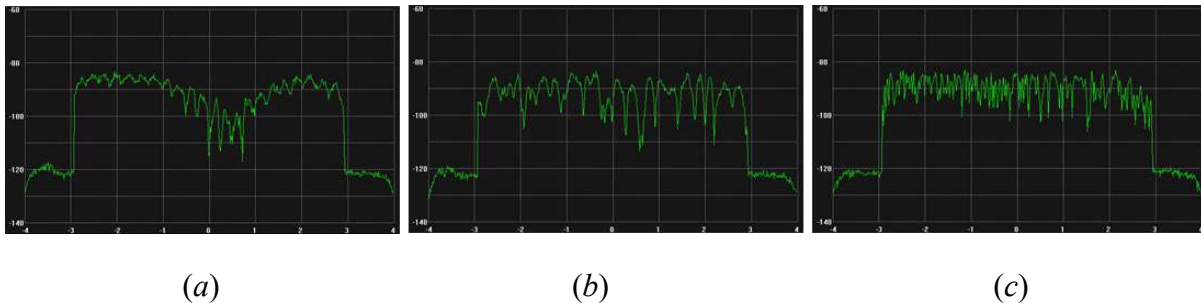
Figure 4.4 Frequency response of a two-transmitter SFN when relative delay is 0.1\ \mu\text{s} : (a) No MISO, (b) MISO with 64 coefficients, and (c) MISO with 256 coefficients
