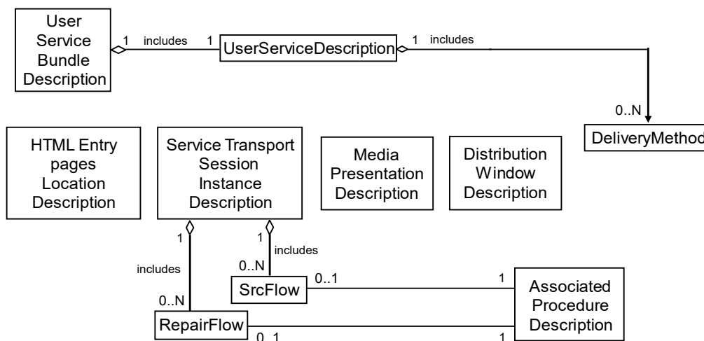
Figure 7.3 Service Layer Signaling data model for ROUTE/DASH Linear Services.
