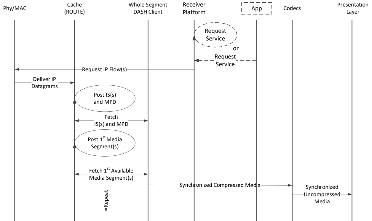
Figure 4.18 Whole segment call flow on receiver.
