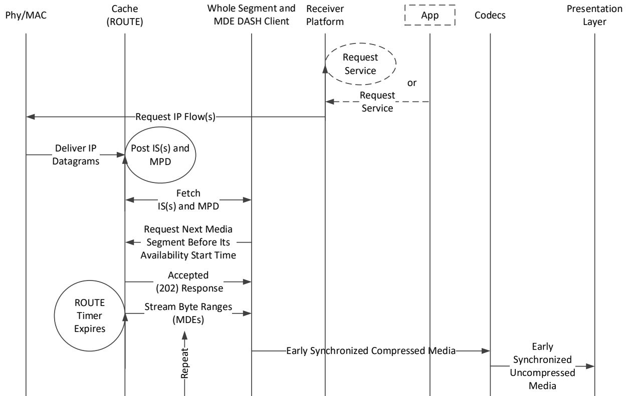
Figure 4.19 MDE delivery call flow.
