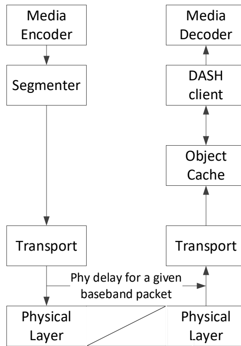
Figure 4.16 Baseband delivery model.
