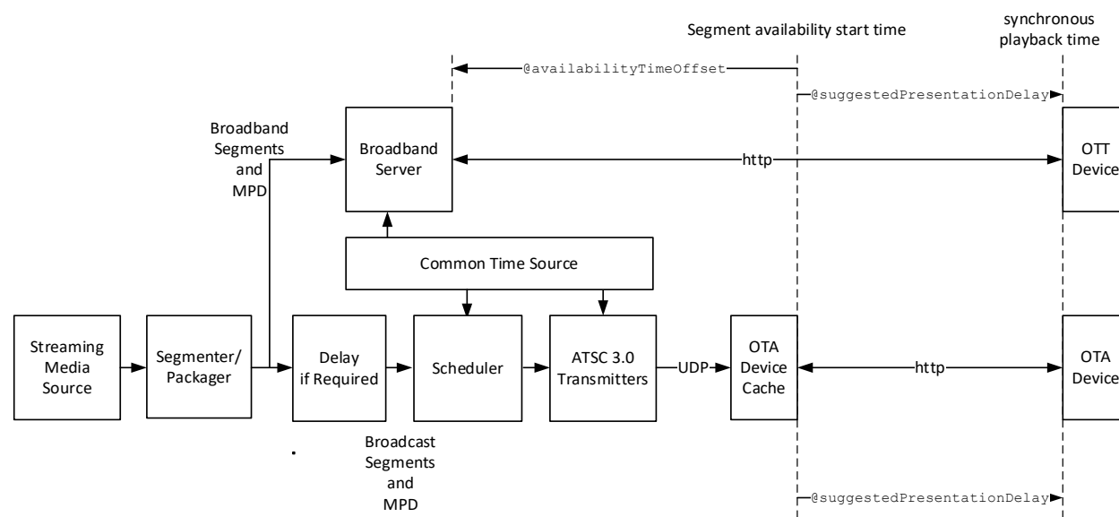
Figure 4.22 DASH attributes and synchronous playback.
