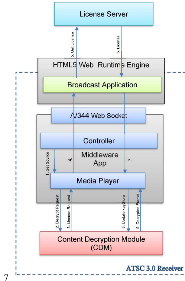
Figure 4-2 A/344 Web Socket workflow.
