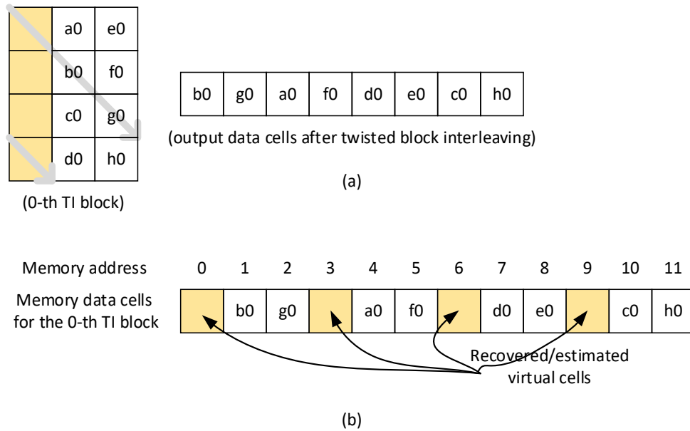
Figure 6.5 Example of time interleaving/de-interleaving with virtual FEC Blocks: (a) Output data cells after TBI operation, (b) Memory data cells after writing into TBI memory.
