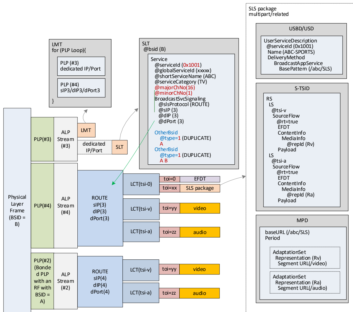
Figure B.16.2 Duplicates of a Service delivered in multiple RF channels with channel bonding (second RF channel).
