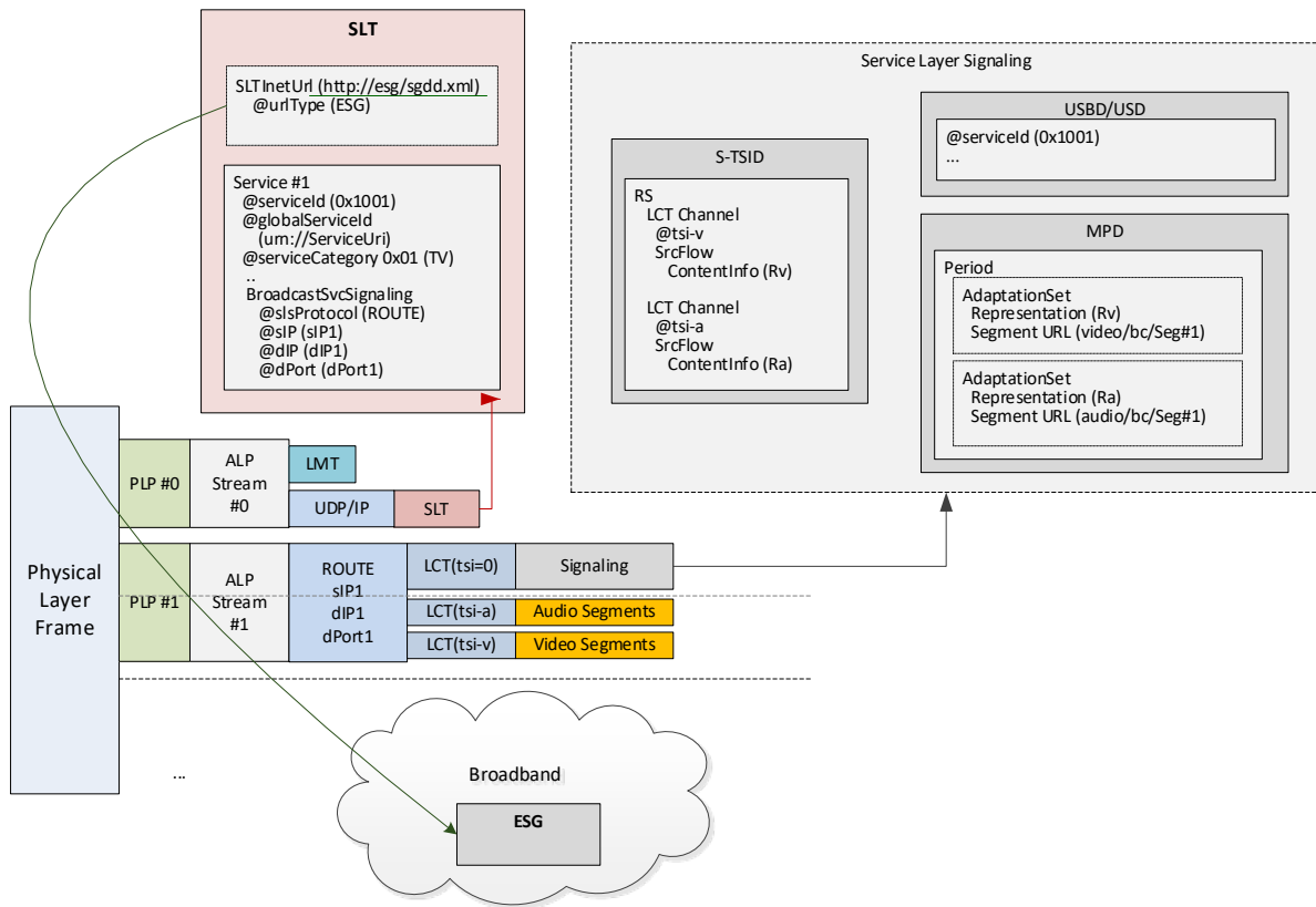
Figure B.6.1 ROUTE ESG bootstrapping via broadband.
