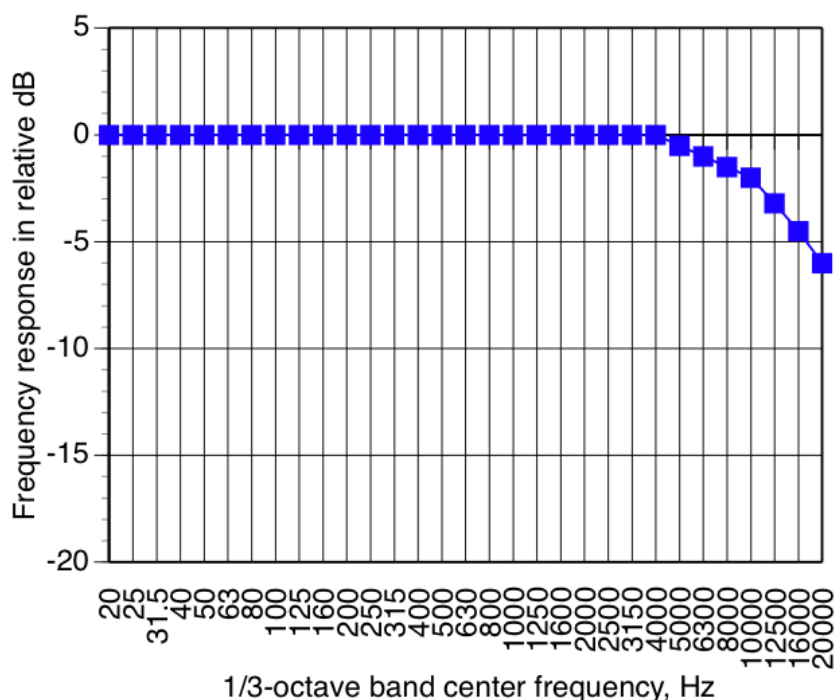
Figure 10.1 Operational room electro-acoustic response curve.
