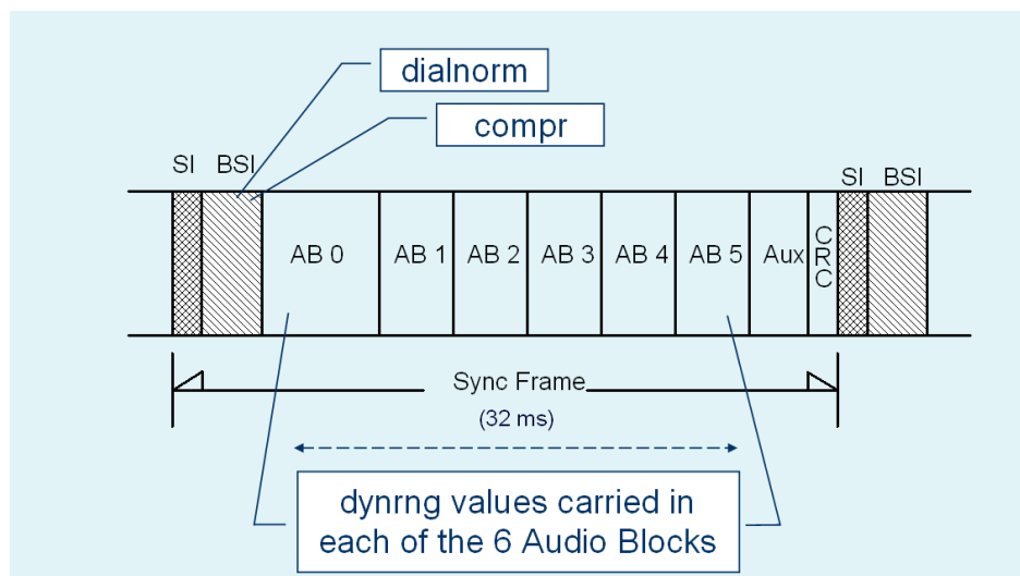
Figure F.4 AC-3 DRC metadata placement in bitstream
