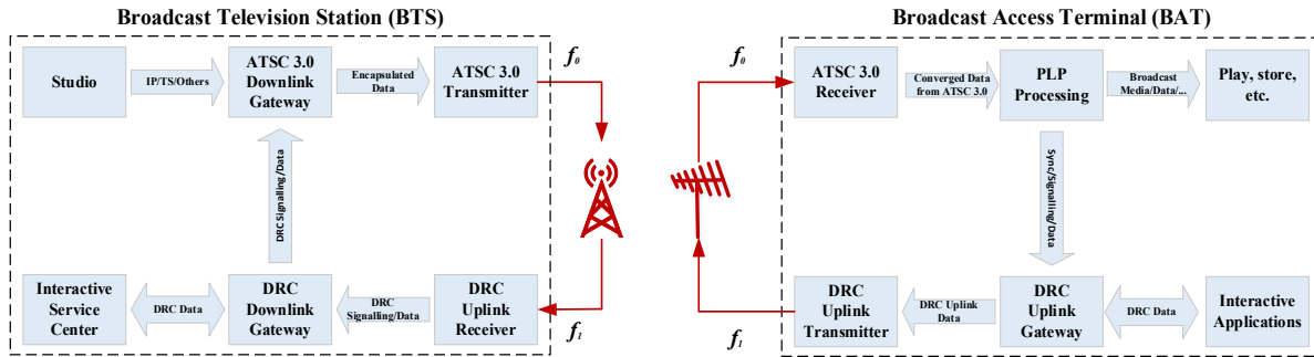
Figure 4.3 System Architecture of ATSC 3.0 with DRC.
