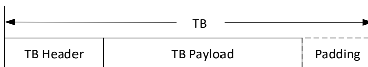
Figure 5.9 Transport Block (TB).
