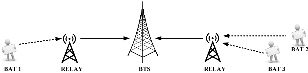
Figure 4.1 Uplink transmission from BATs to BTS through relays.
