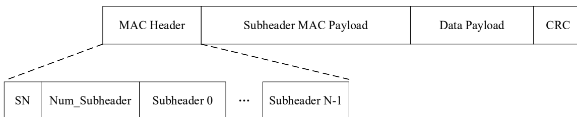
Figure 6.6 Structure of Uplink MAC PDU.
