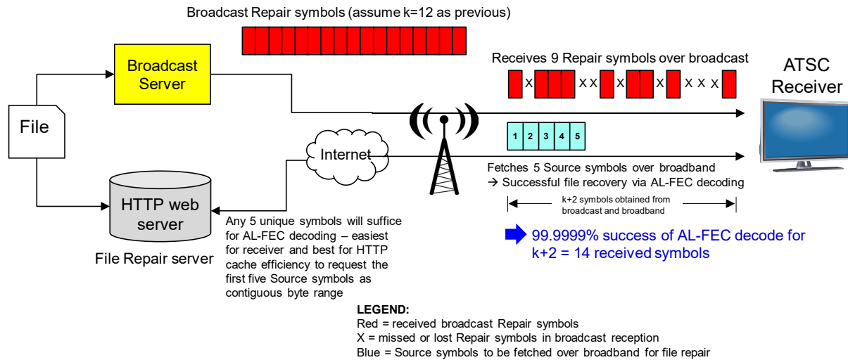
Figure 4.15 Transmission of strictly repair data.
