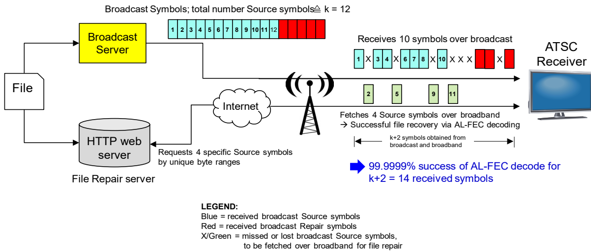
Figure 4.14 Transmission of source followed by repair data.
