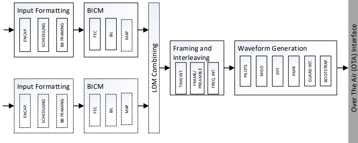
Figure 6.14 Block diagram of LDM encoding.
