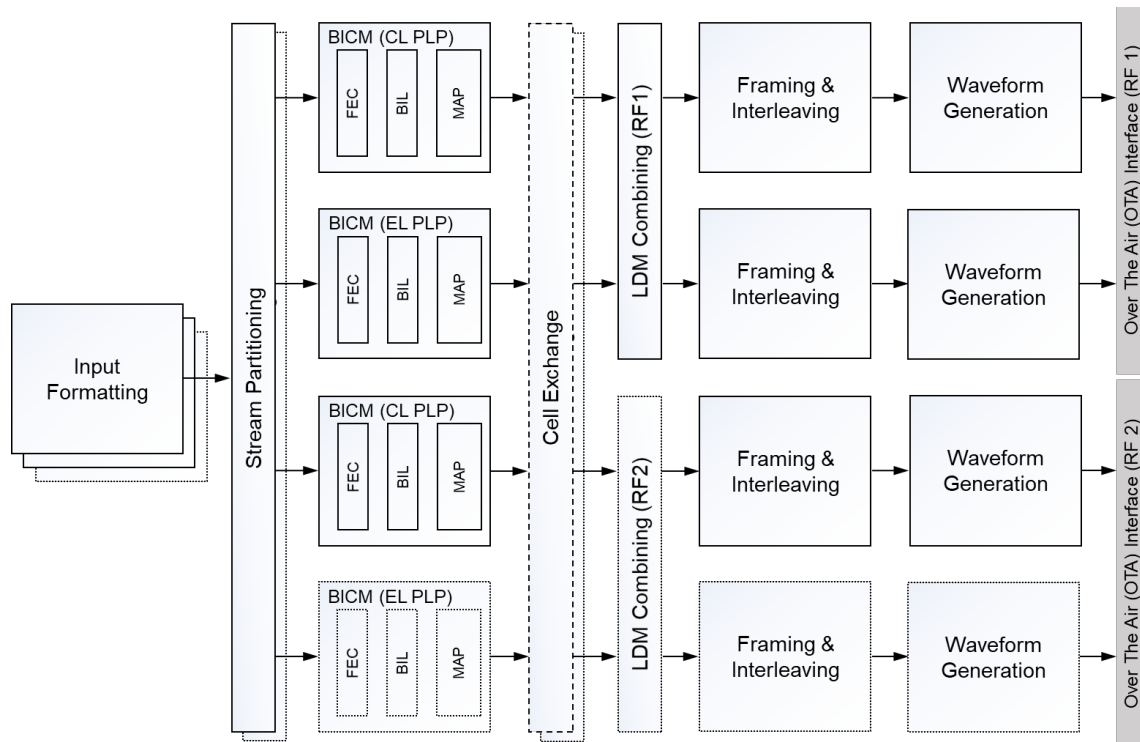
Figure K.4.1 Block diagram of channel bonding with LDM.
