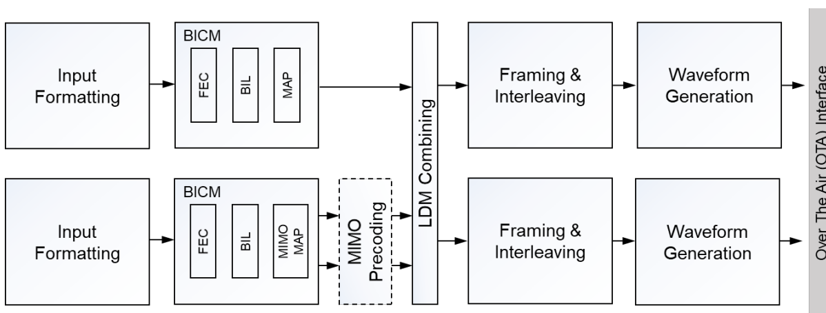
Figure O.1.3 Block diagram of Layered MIMO Type B.
