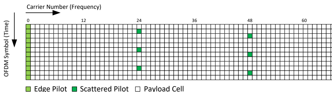
Figure E.1.14 Scattered pilot pattern SP24_4 (SISO, D_X = 24 , D_Y = 4 ).
