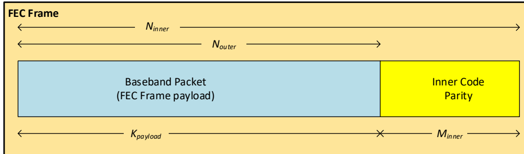
Figure 6.3 Structure of FEC Frame when no Outer Code is used.
