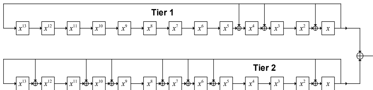
Figure N.2.4 TxID code generator based on Gold sequence.
