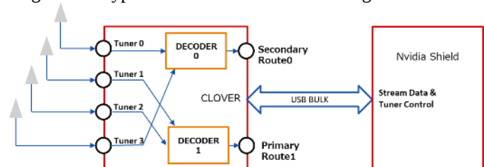
Figure VI.1 CXD2885GG Configuration
