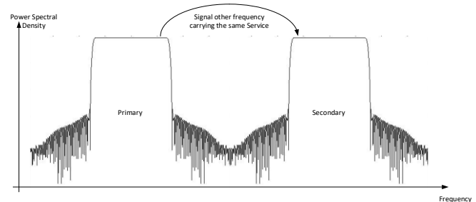
Figure II.2 MFN Signaling
