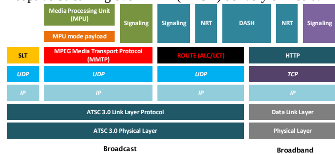
Figure II.1 ATSC 3.0 Protocol Stack
