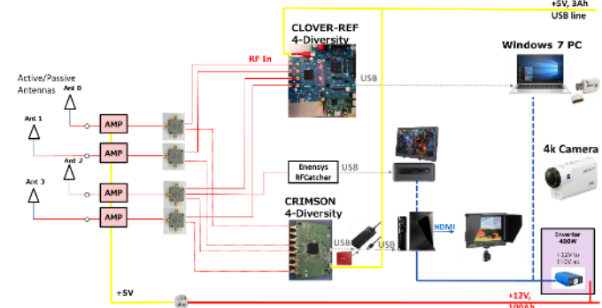
Figure VI.2 Field test wiring diagram
