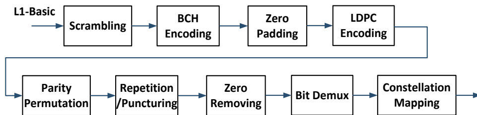
Figure 6.18 Block diagram of L1-Basic protection.
