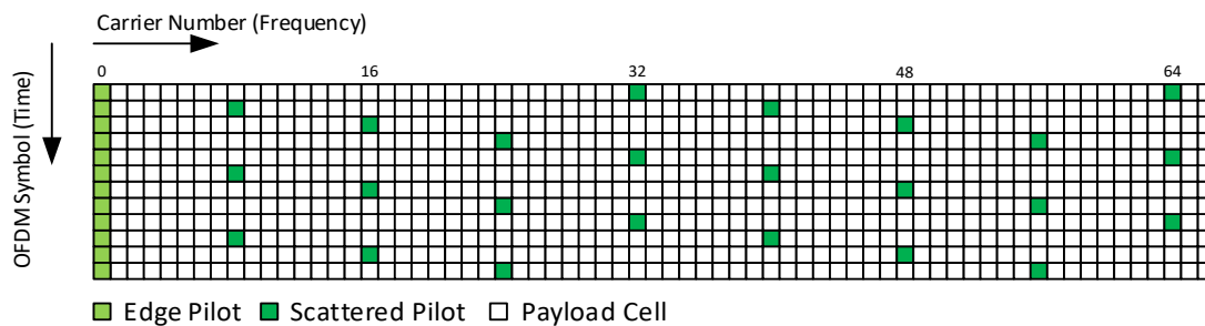
Figure E.1.8 Scattered pilot pattern SP8_4 (SISO, D_X = 8 , D_Y = 4 ).
