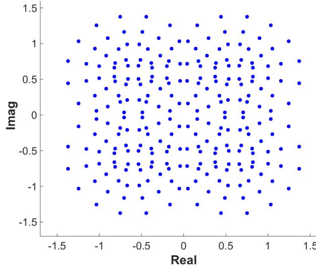
Figure 6.17 Example combined constellation after normalization.
