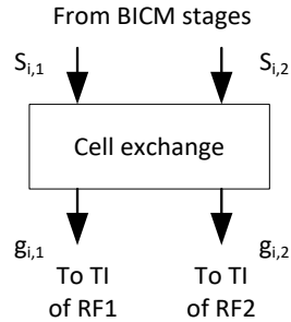
Figure K.3.1 Cell exchange block.
