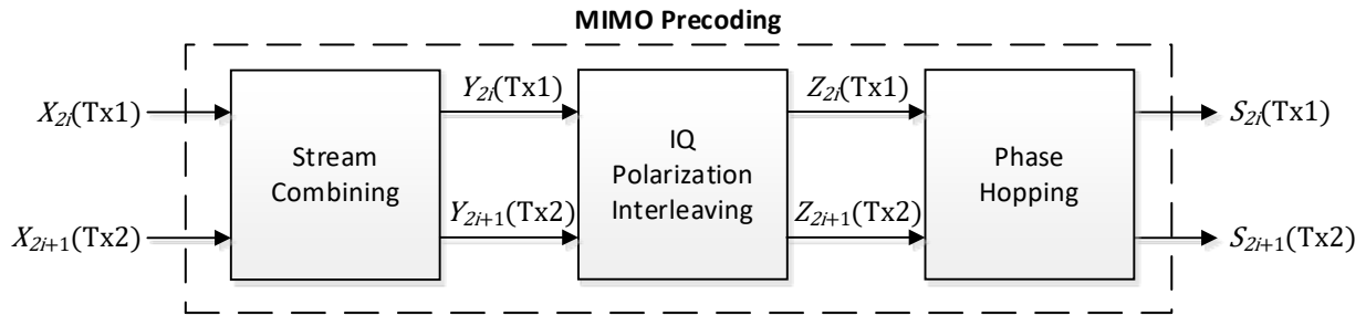
Figure L.5.2 Detailed MIMO precoding block diagram.
