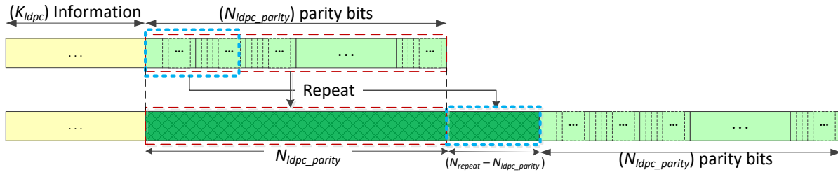
Figure 6.23 Parity Repetition ( N_{repeat} > N_{ldpc\_parity} ).
