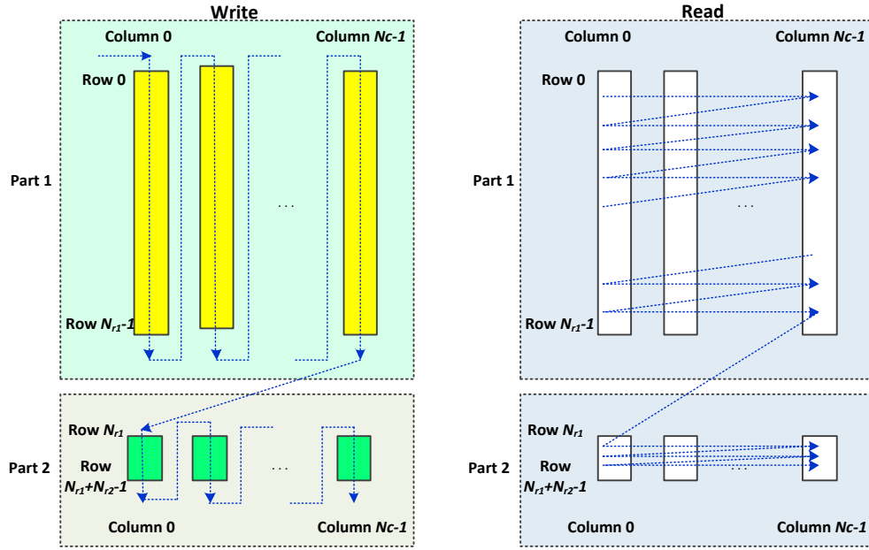
Figure 6.7 Write/Read operation of Type A block interleaving.
