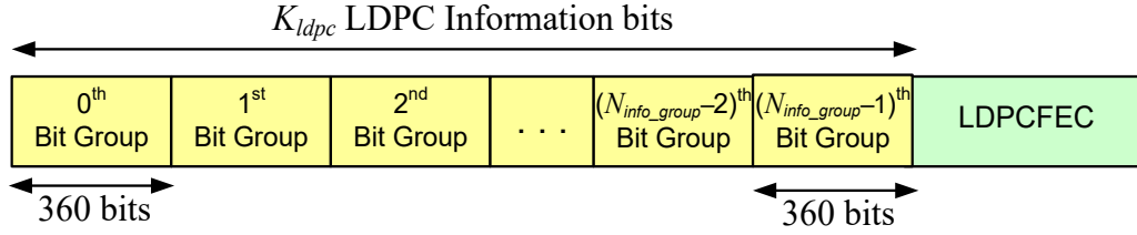
Figure 6.20 Format of data after LDPC encoding of L1-Basic/-Detail signaling.
