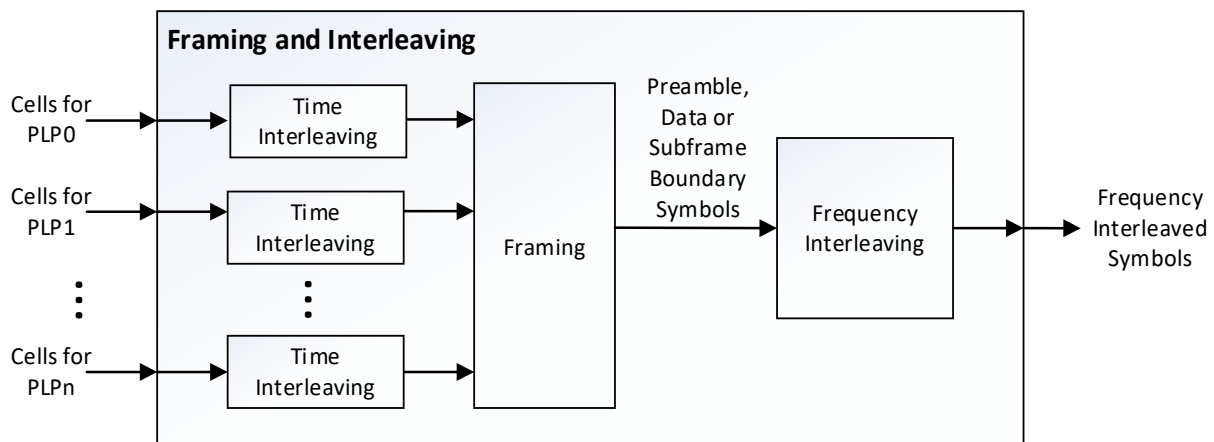
Figure 7.1 Block diagram of framing and interleaving.
