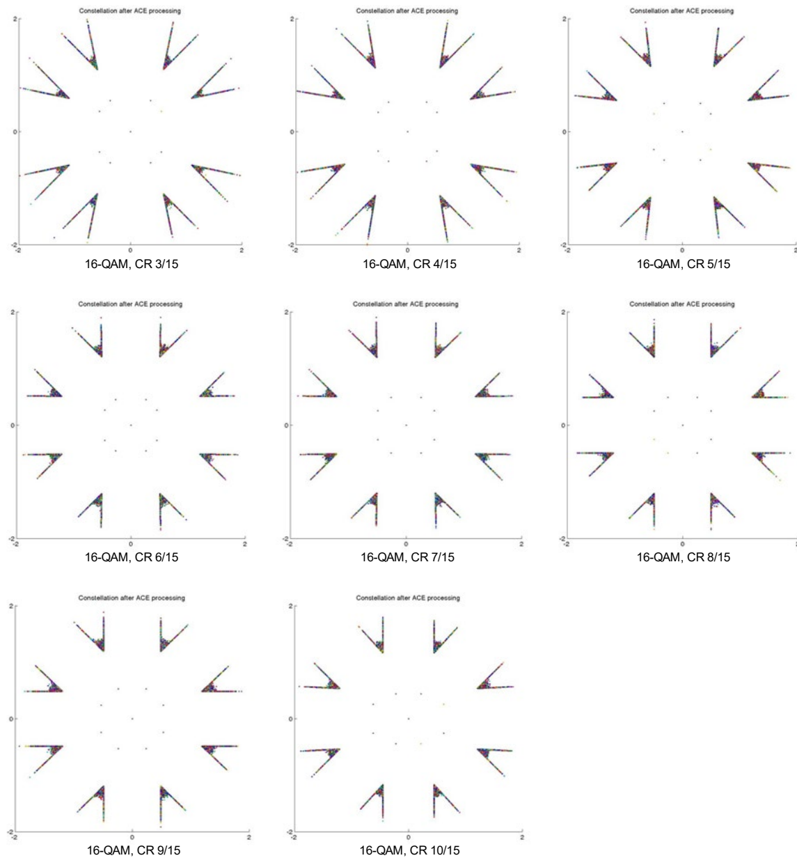
Figure M.3.3 Constellation diagram for 16QAM when using the defined ACE algorithm.
