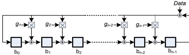
Figure 6.4 Shift register for CRC-32.
