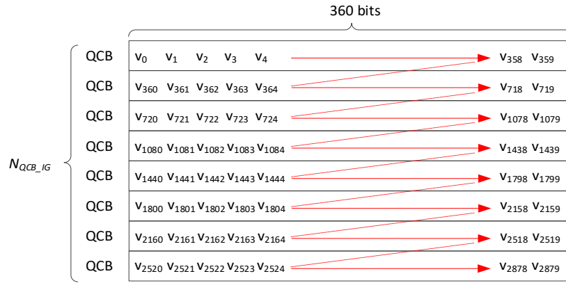
Figure 6.8 Write operation of Part 1 Type B block interleaving for 256QAM.
