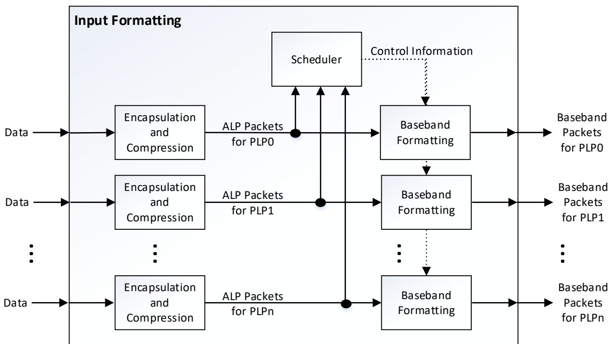
Figure 5.1 Block diagram of input formatting.
