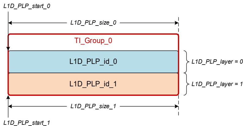
Figure 7.18 LDM Example #1 (1 Core PLP, 1 Enhanced PLP).
