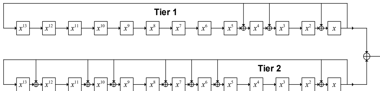
Figure N.2.4 TxID code generator based on Gold sequence.
