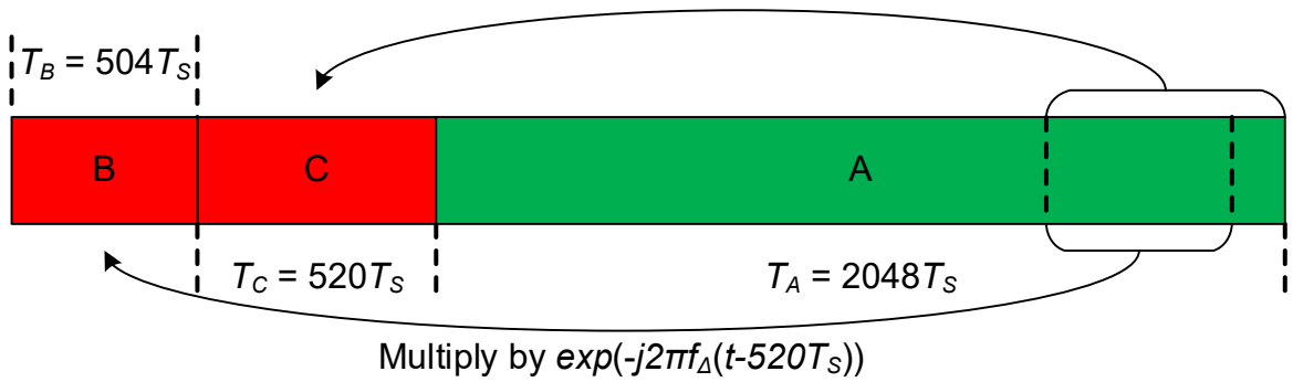
Figure 5.6 BCA time domain symbol structure.
