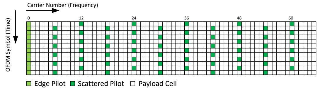
Figure E.1.5 Scattered pilot pattern SP6_2 (SISO, D_X = 6 , D_Y = 2 ).
