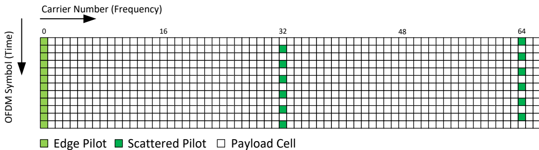
Figure E.1.15 Scattered pilot pattern SP32_2 (SISO, D_X = 32 , D_Y = 2 ).
