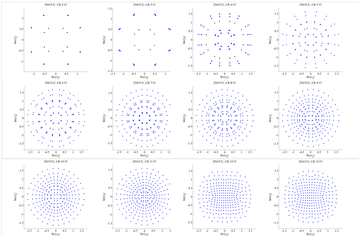
Figure C.2.4 Constellations of 256QAM.
