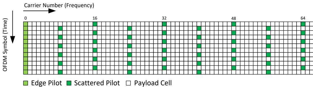
Figure E.1.7 Scattered pilot pattern SP8_2 (SISO, D_X = 8 , D_Y = 2 ).
