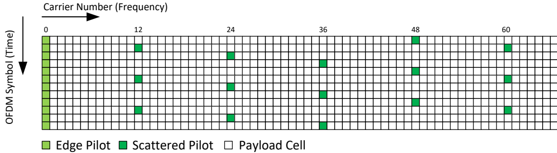
Figure E.1.10 Scattered pilot pattern SP12_4 (SISO, D_X = 12 , D_Y = 4 ).
