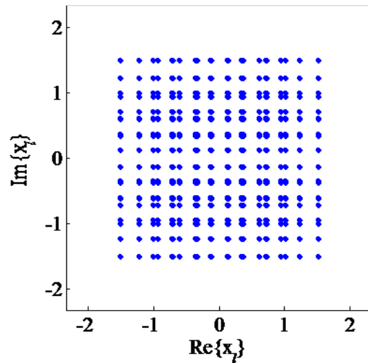
Figure 6.13 Example 1024-NUC for code rate 6/15.
