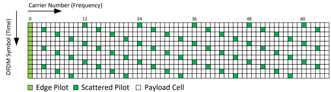
Figure E.1.2 Scattered pilot pattern SP3_4 (SISO, D_X = 3 , D_Y = 4 ).
