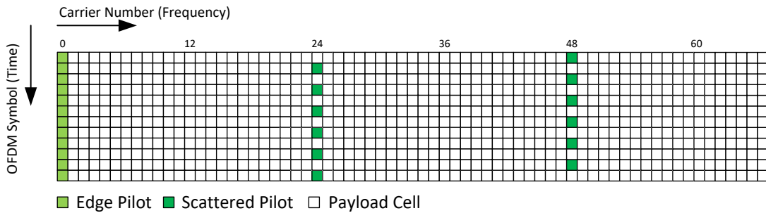
Figure E.1.13 Scattered pilot pattern SP24_2 (SISO, D_X = 24 , D_Y = 2 ).
