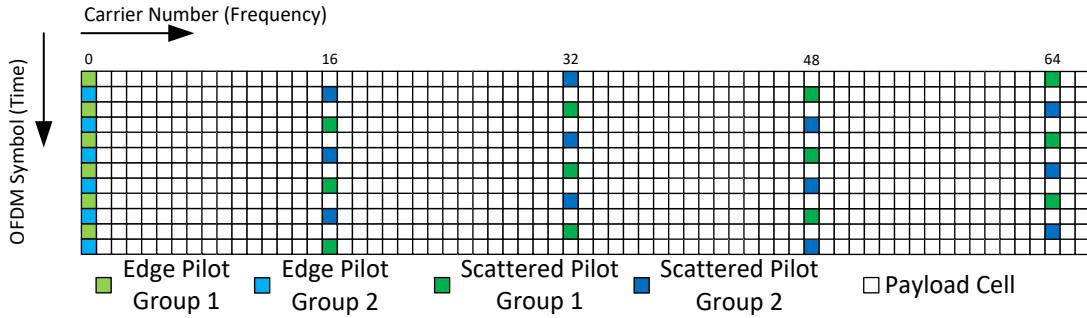
Figure L.9.23 MIMO pilot scheme MP16_2 for null pilot encoding.
