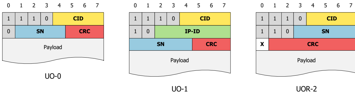
Figure C.2.3 Compressed IP packet format (Small CID, CID ≠ 0)
