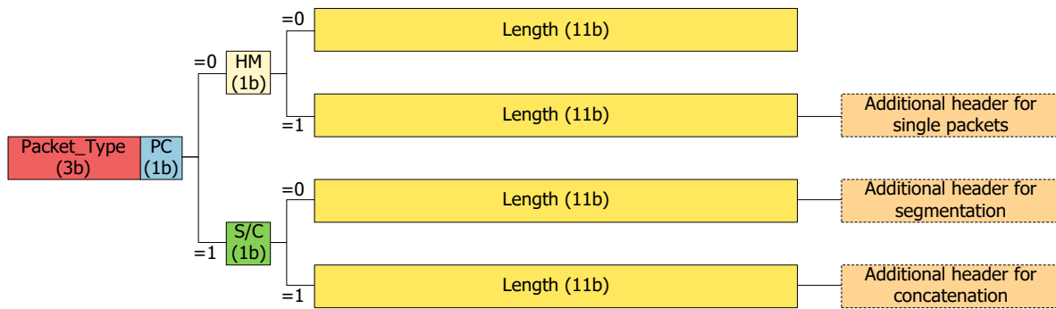
Figure 5.2 Structure of Base Header for ALP packet encapsulation.
