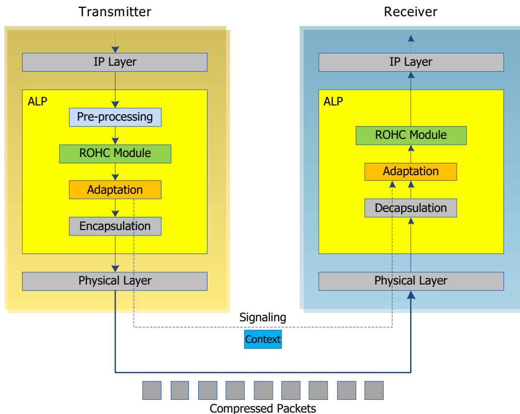
Figure 6.1 Functional structure of IP header compression and decompression.
