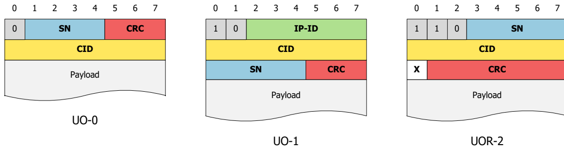
Figure C.2.6 Compressed IP packet format (Large CID)
