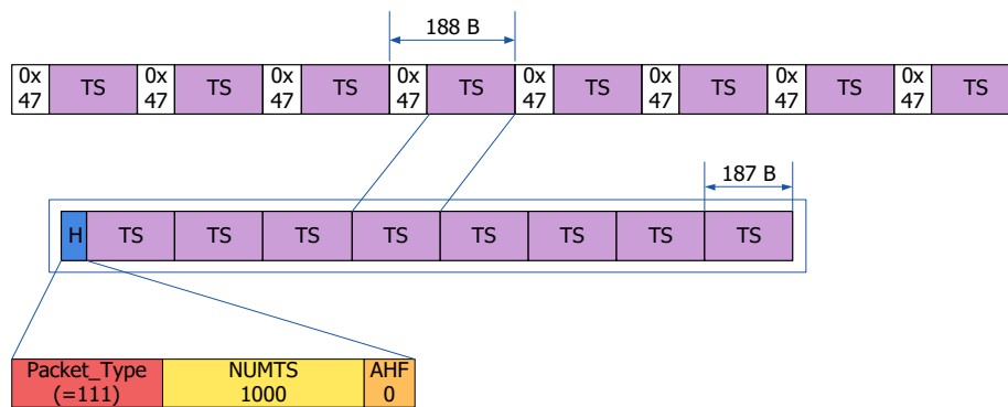
Figure B.2.1 MPEG-2 TS encapsulation example.
