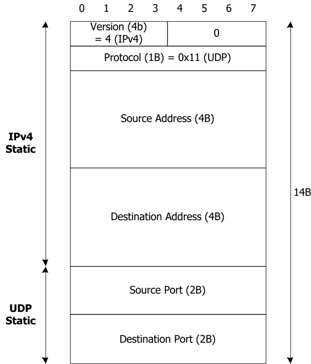
Figure C.1.1 Format of static chain
