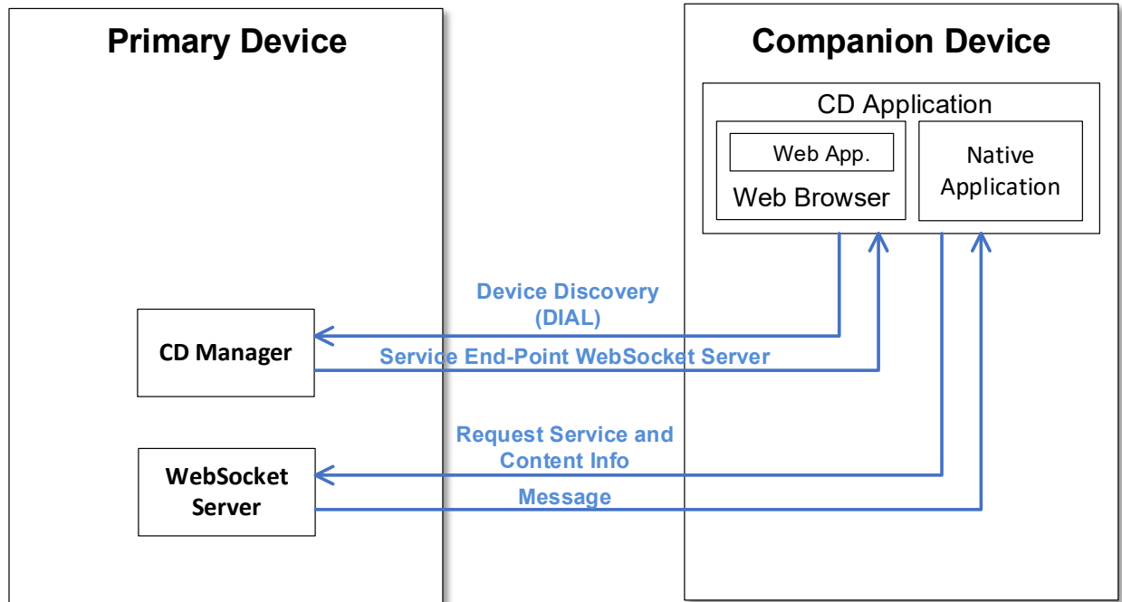
Figure 5.3 Architecture for CD Application to PD communication.
