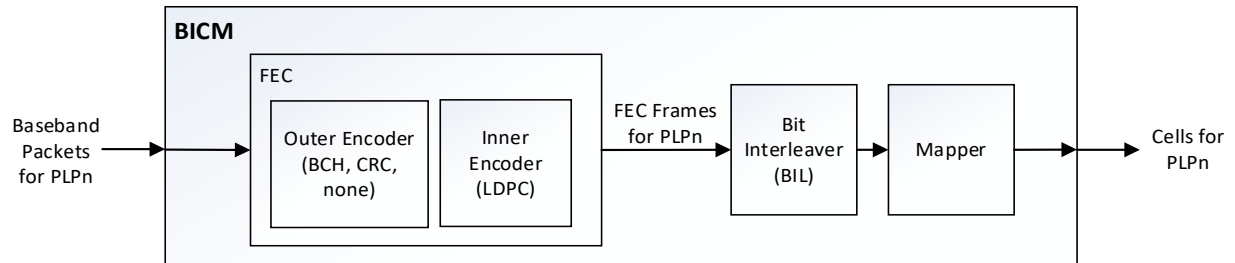
Figure 6.1 Block diagram of BICM.
